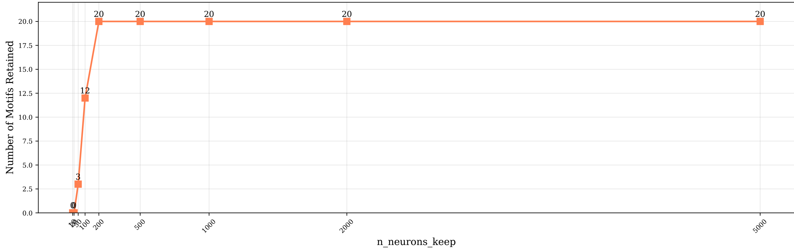
Motif Retention vs Neuron Threshold sigma: (0.02, 0.4) | volume: (0.02, 0.9)
